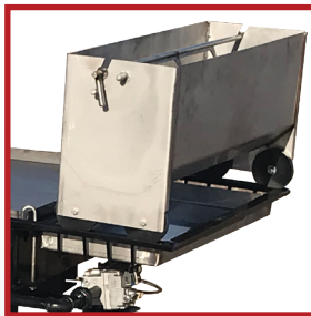
Batter dispenser sitting over the drip pan area
