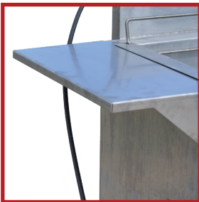
Two side shelves: 14" L x 26" W
